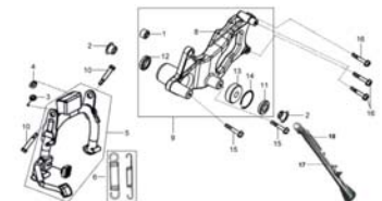
F12 MAIN STAND & RR. FORK
