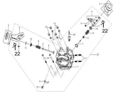
E05 CYLINDER
