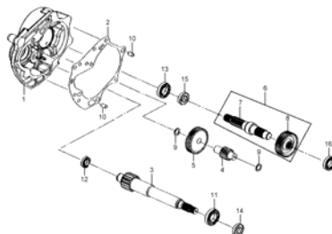
E11 MISSION CASE & DRIVE SHAFT
