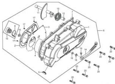
E11 MISSION CASE & DRIVE SHAFT
