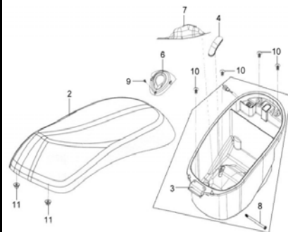
F12 DOUBLE SEAT LUGGAGE BOX
